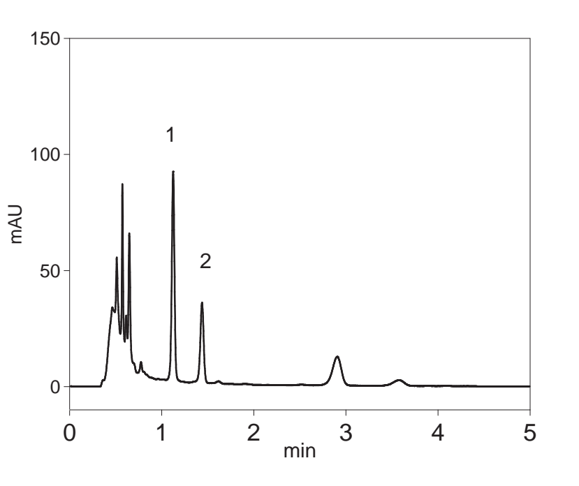
benzoic acid
